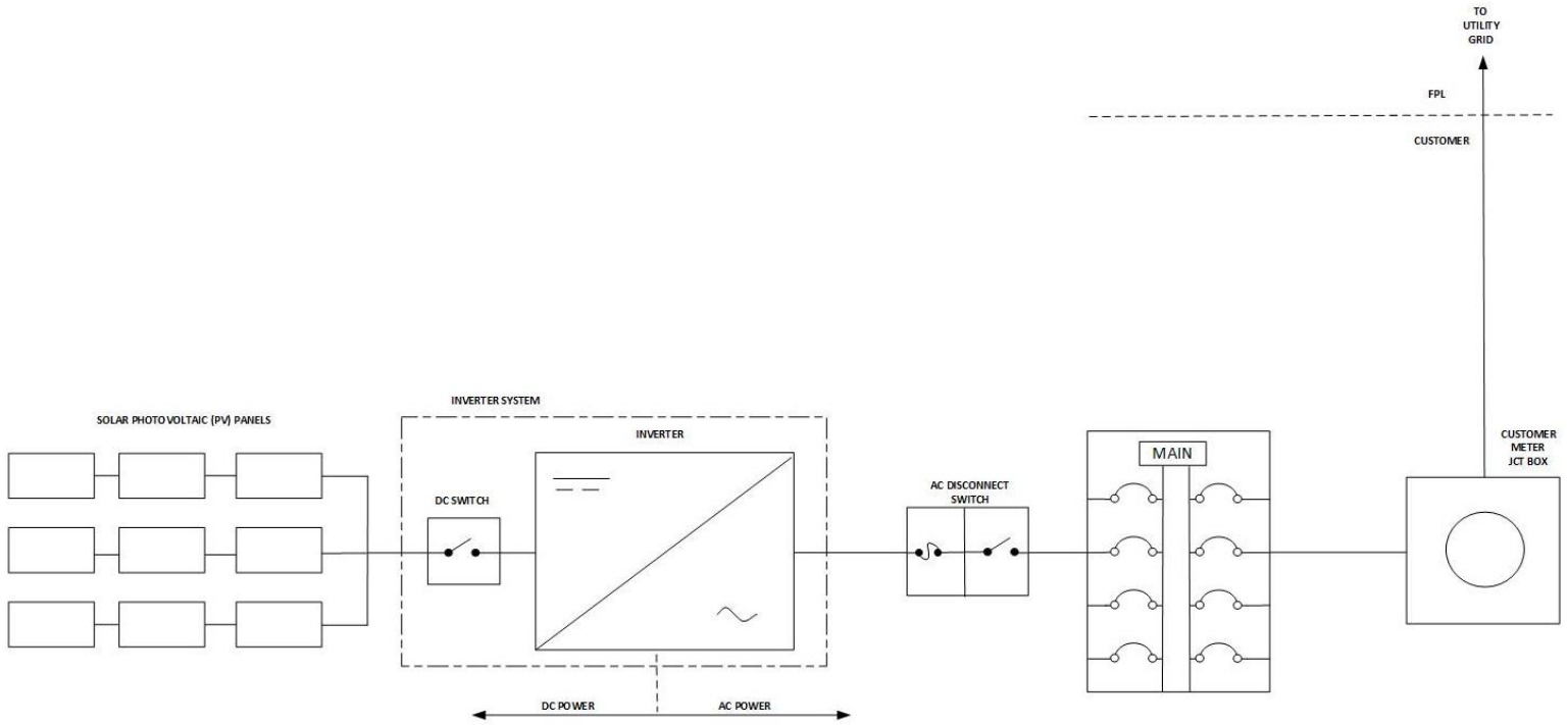
FIGURE IV-1 Net Metering (Conceptual Drawing)
