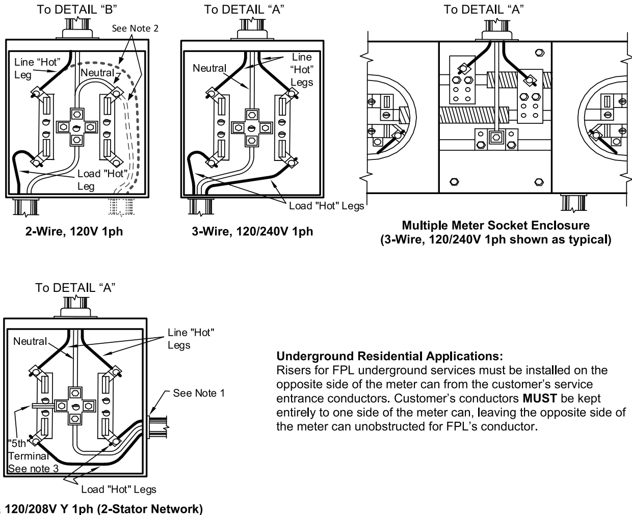
FIGURE IV-8a Self-Contained Meter Installation – Residential Overhead Service (200A or less)
